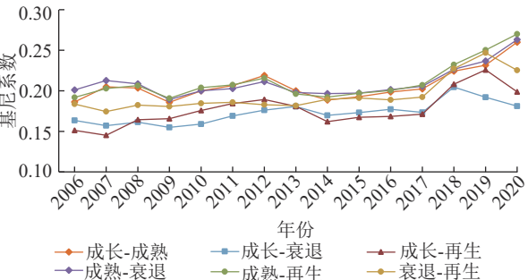
图 8 不同成长阶段资源型城市的区域间差异变化趋势 Fig. 8 The trend of regional differences in land green use efficiency in resource-based cities at different growth stages
